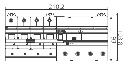
4 POLE (12 MOD)
