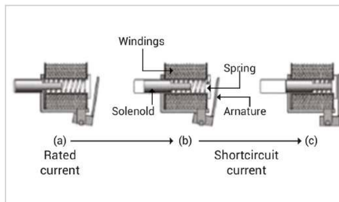
Solenoid
