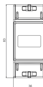
1-PhaseMeter
