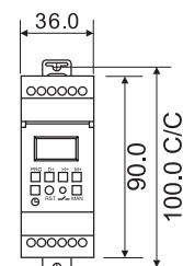
ASTRO / DIGITAL
