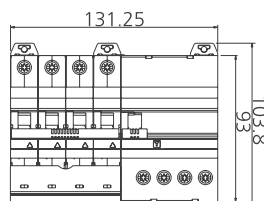
4 POLE (7.5 MOD)
