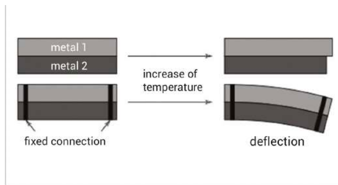
Bimetallic strip
