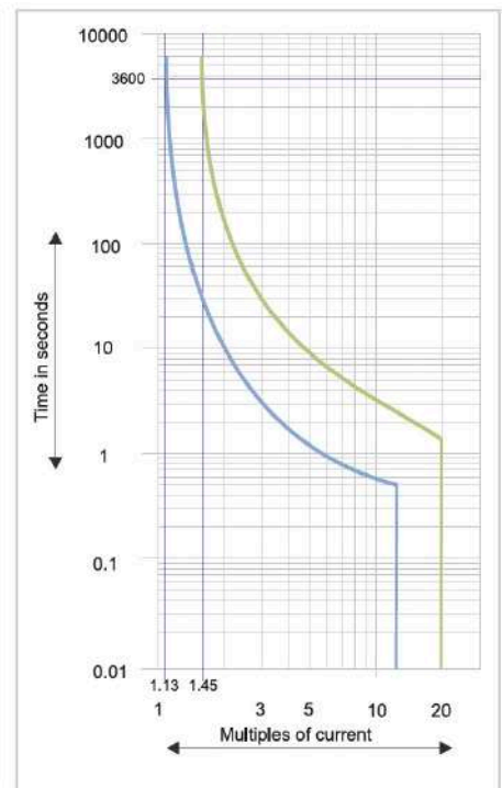
E Curve
