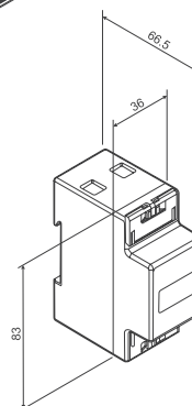
1-PhaseMeter
