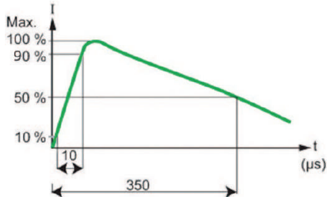
10/350 microsecond waveform
